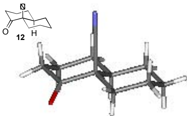
Structure of 12 (R=0.044)
