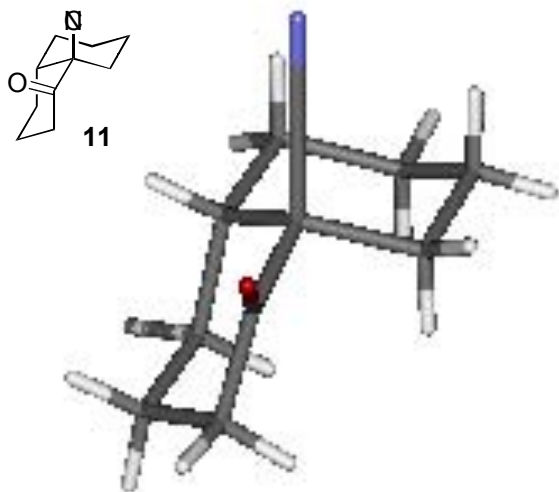
Structure of 11 (R=0.040)
